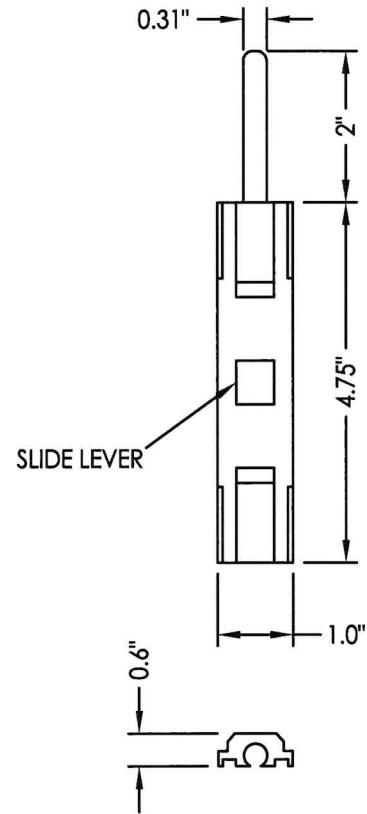
SLIDE BOLT ASSEMBLY w/ Slide Lever (PVC)
