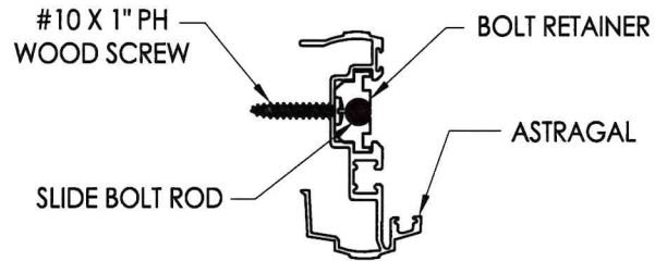
SECTION A-A Astragal Assembly
