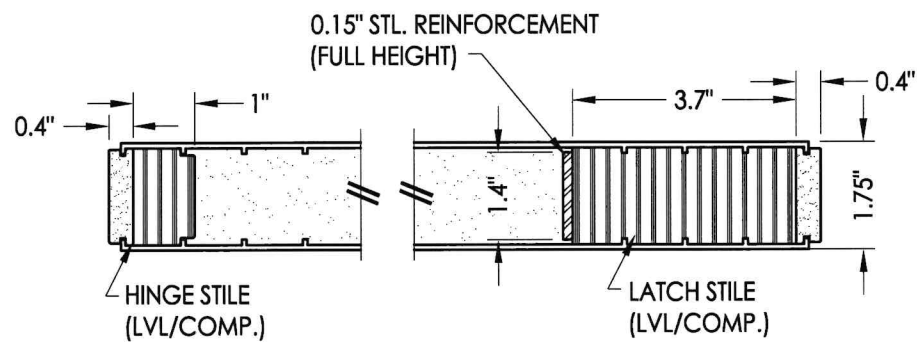
SECTION C-C
