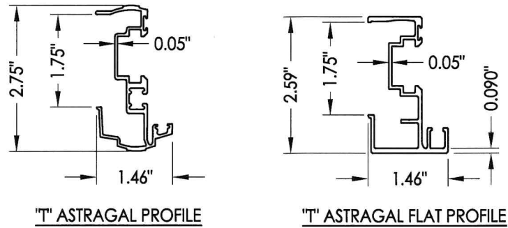
16 "ALUMINUM "T" ASTRAGAL by AFCO
