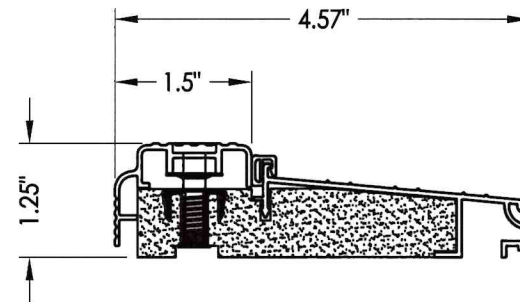
11 INSWING THRESHOLD AFCO A-276
